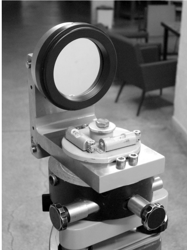
Photo 3. Reflecting device on measuring post
