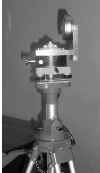
Photo 6. Reflection device in the process of breaking the level aiming line
