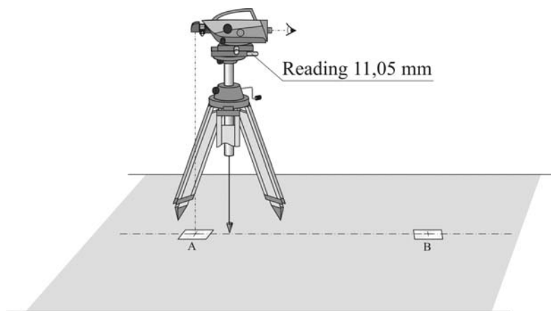
Fig. 3. Stage II – setting the level with the stage over the beginning of the measured sector and performing the second reading on the micrometric screw of the stage.
