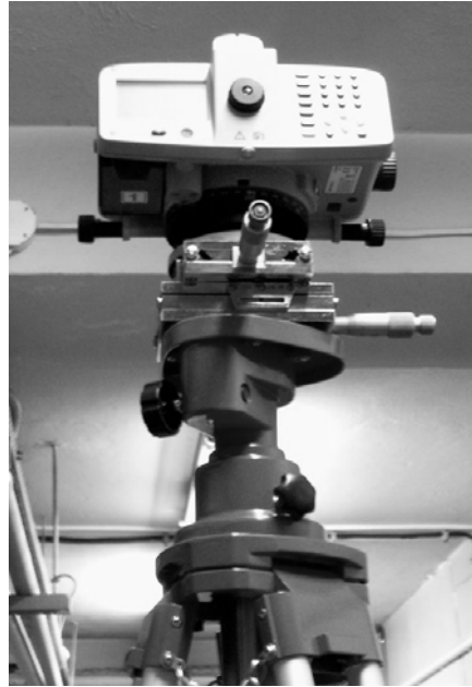
Photo 4. View of instrument placed on micrometric stage
