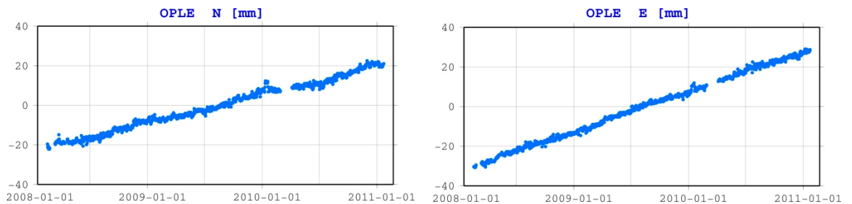
Fig. 8 Time series of OPLE (Opole, PL) GPS site.
